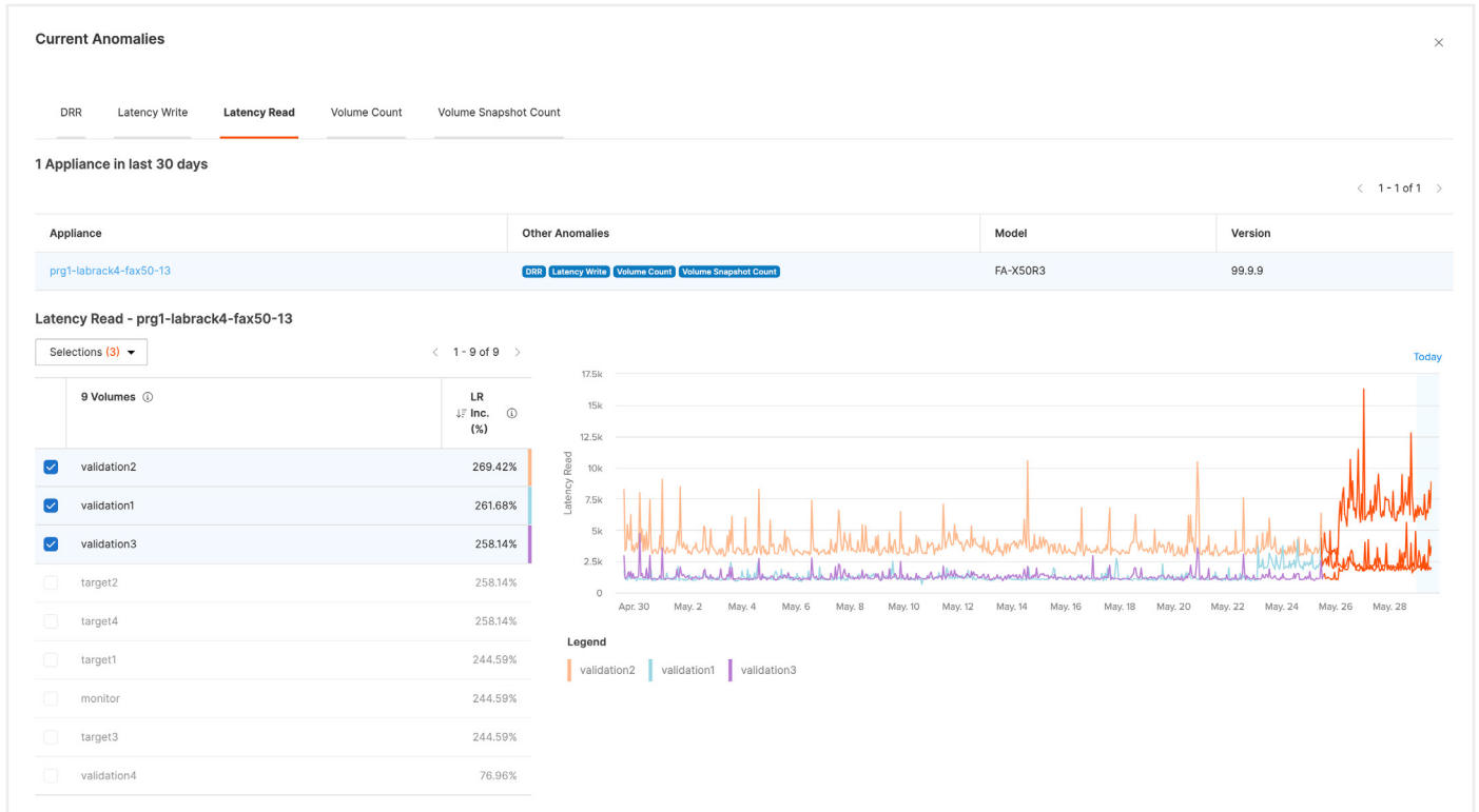
FIGURE 1 Anomaly Detection in Pure1
